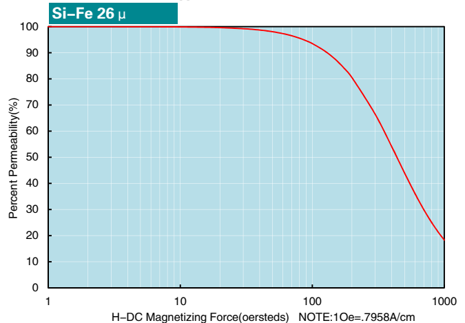
DC-Bias Curves(Typical)
